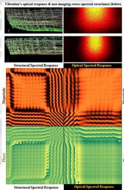
Tank armor nonlinear clattering sensed by laser imaging. Time evolution of modes analyzed for covariance of the spectra, structural vs. optical.
